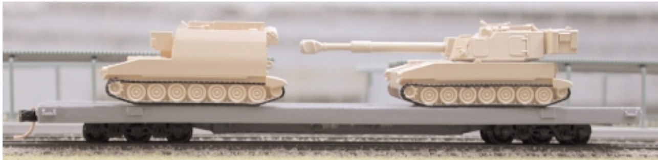
Pilot model of 150 ton flat car (un-painted) shown with production versions of M992 and Paladin.
